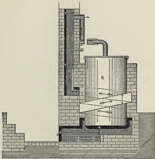
FIG. 5.—Set-kettle for Varnish. The grate is on wheels, by which the fire may be withdrawn.
